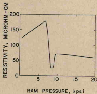
FIG. 9. The resistivity of bismuth as a function of ram pressure. This curve was derived from the observed data of Fig. 8.
