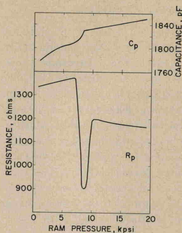
FIG. 10. Directly observed parallel tuning capacitance and equivalent parallel resistance of coil on filamentary bismuth core. In this case the skin depth is equal to the effective sample radius.
