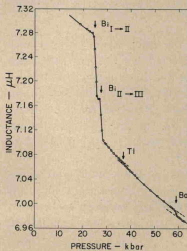
FIG. 11. The inductance of the coil on a compound core of concentric cylinders of bismuth (80%), thallium (10%), and barium (10%).
