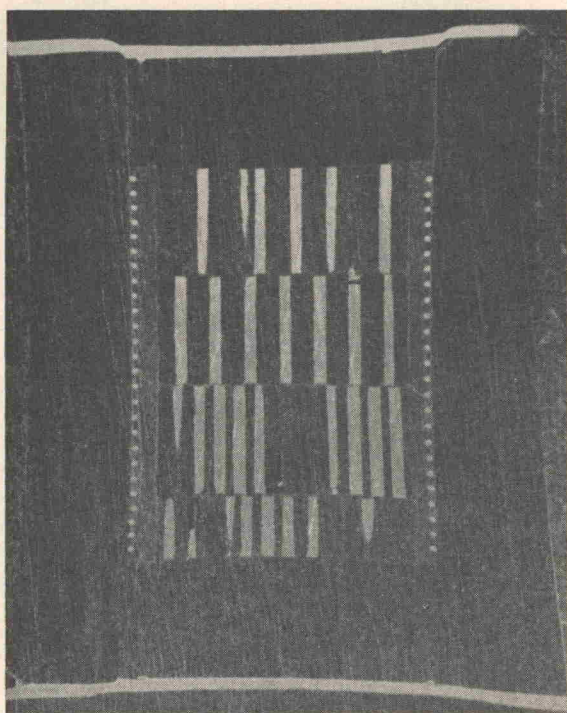
FIG. 5. Cross section of the filamentary sample core for which the skin depth equals the radius of the bismuth needles.
