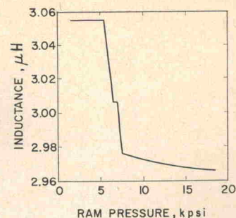
FIG. 6. Inductance of a standard sample coil on a bismuth core at 1000 cps. The skin depth in this case is much larger than the core dimensions.
