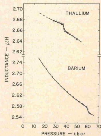
FIG. 7. Inductance of coil on barium and thallium cores at 1000 cps.
