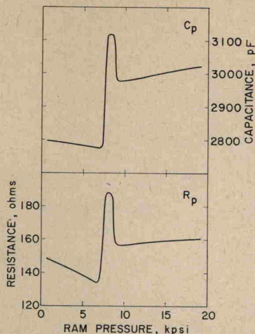
FIG. 8. Directly observed parallel impedance of coil on a bismuth core at 2.1 Mc. The skin depth here is much less than the dimensions of the core.
